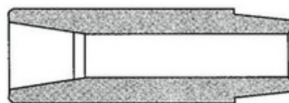
图2-1(Fig.2-1) 代用接头(Cross-Over Sub)
