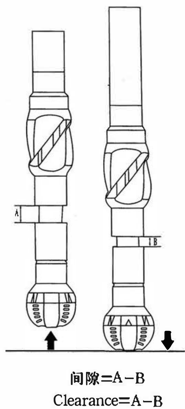
最大允许轴向轴承间隙说明:见图表2 Allowed Maximal Clearance of Axial Bearing:(see Table.2)
